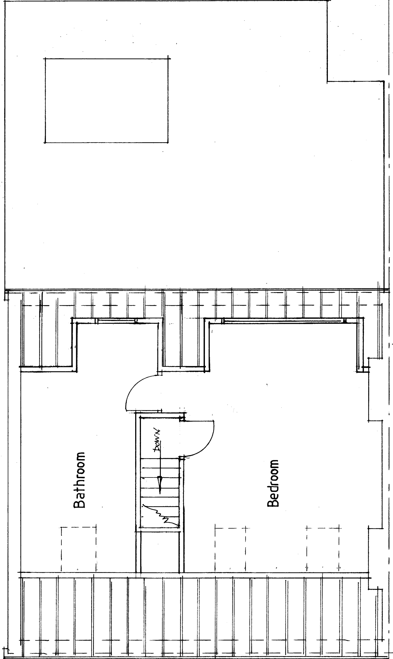
Loft Plan - proposed
