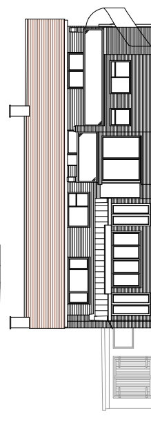
SOUTH ELEVATION 1:100
