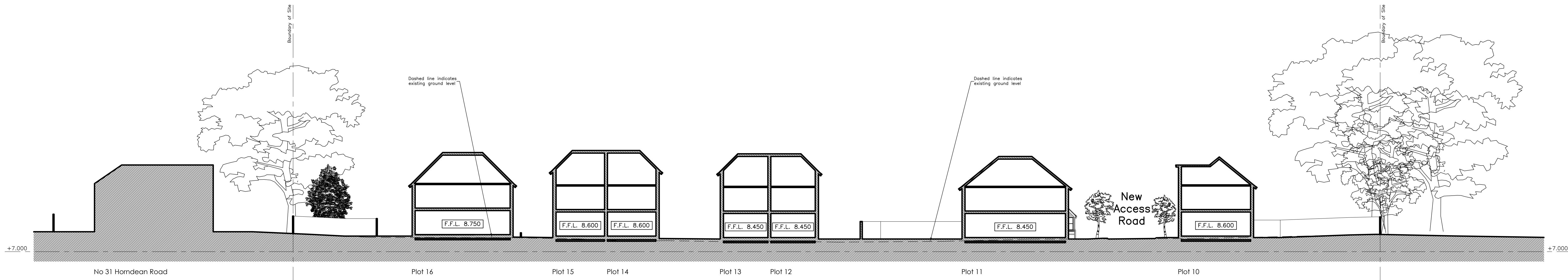
Longitudinal Section Through Central Part of Site (From Plot 16 through to Plot 10)
