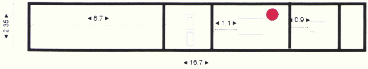
Left Elevation
