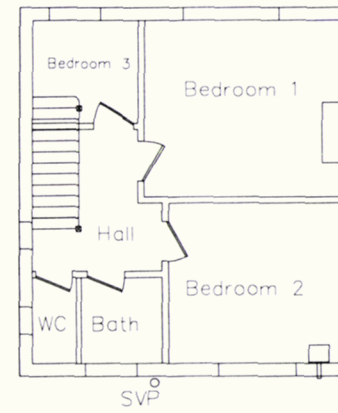
First Floor Layout
