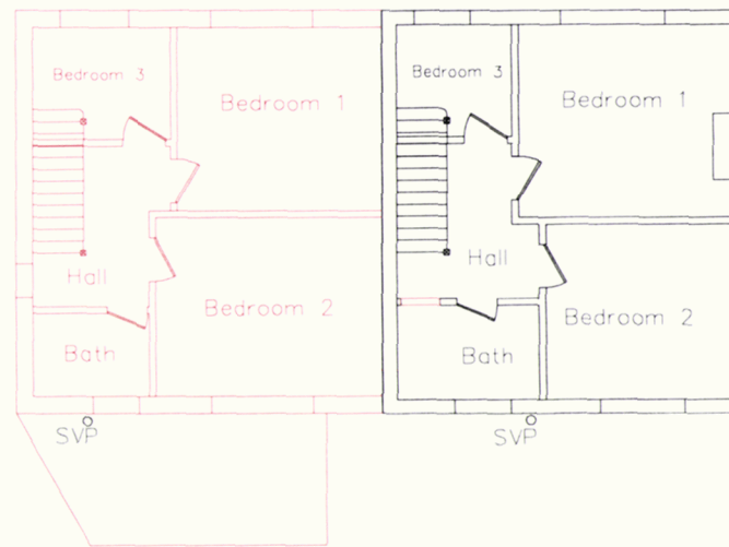
Proposed First Floor Layout
