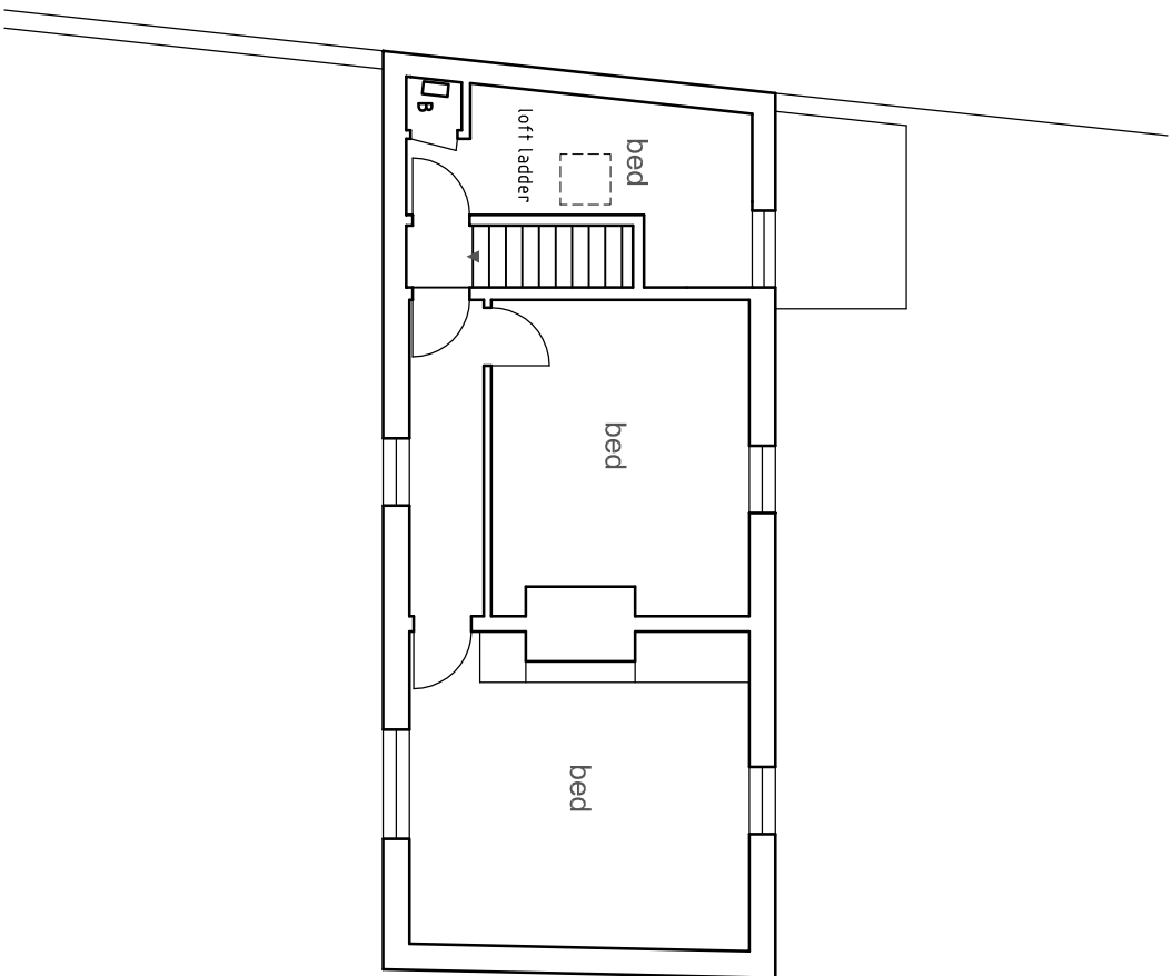
FIRST 1:100
