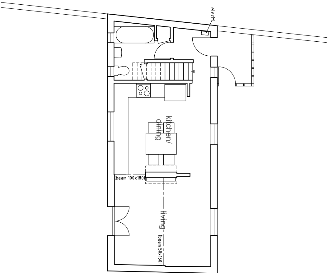
GROUND 1:100
