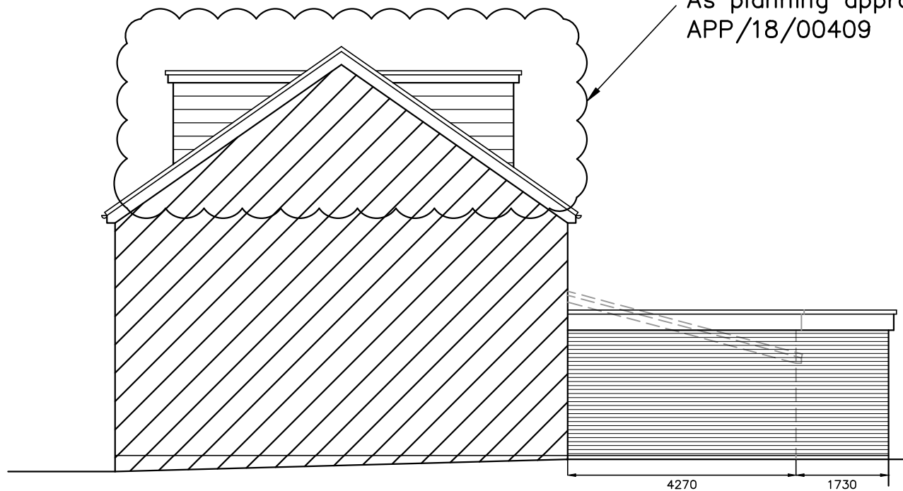
West Elevation
