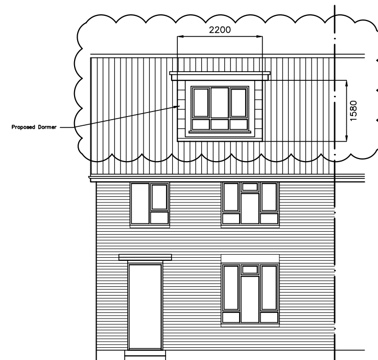
North Elevation
