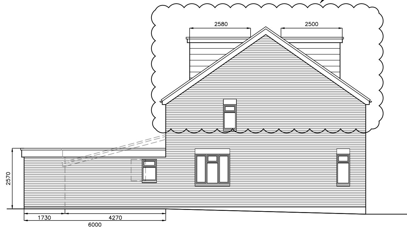
East Elevation
