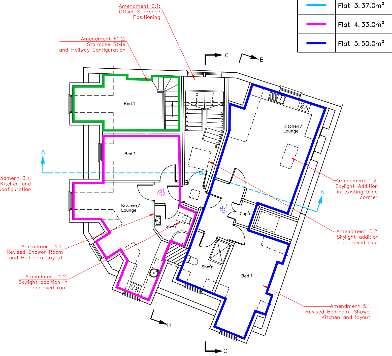
SECOND FLOOR
