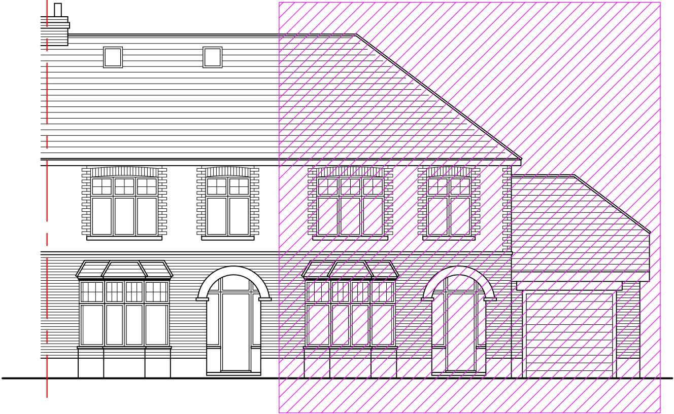
PROPOSED NORTH (FRONT) ELEVATION
