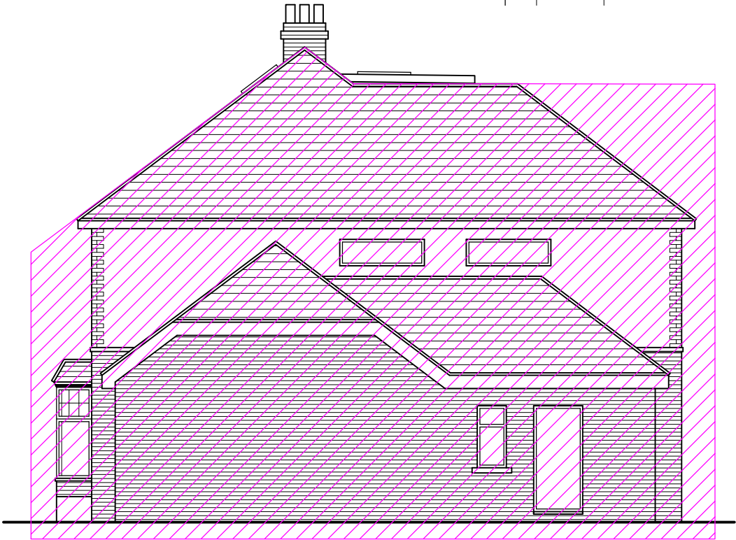
PROPOSED WEST (SIDE) ELEVATION
