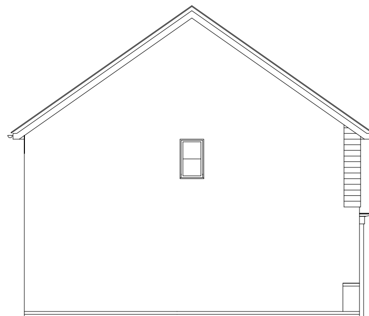
SIDE ELEVATION 1
