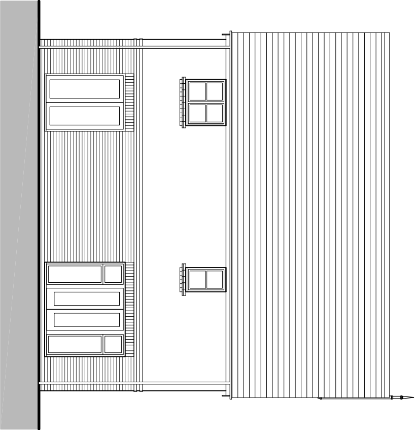
REAR ELEVATION - C
