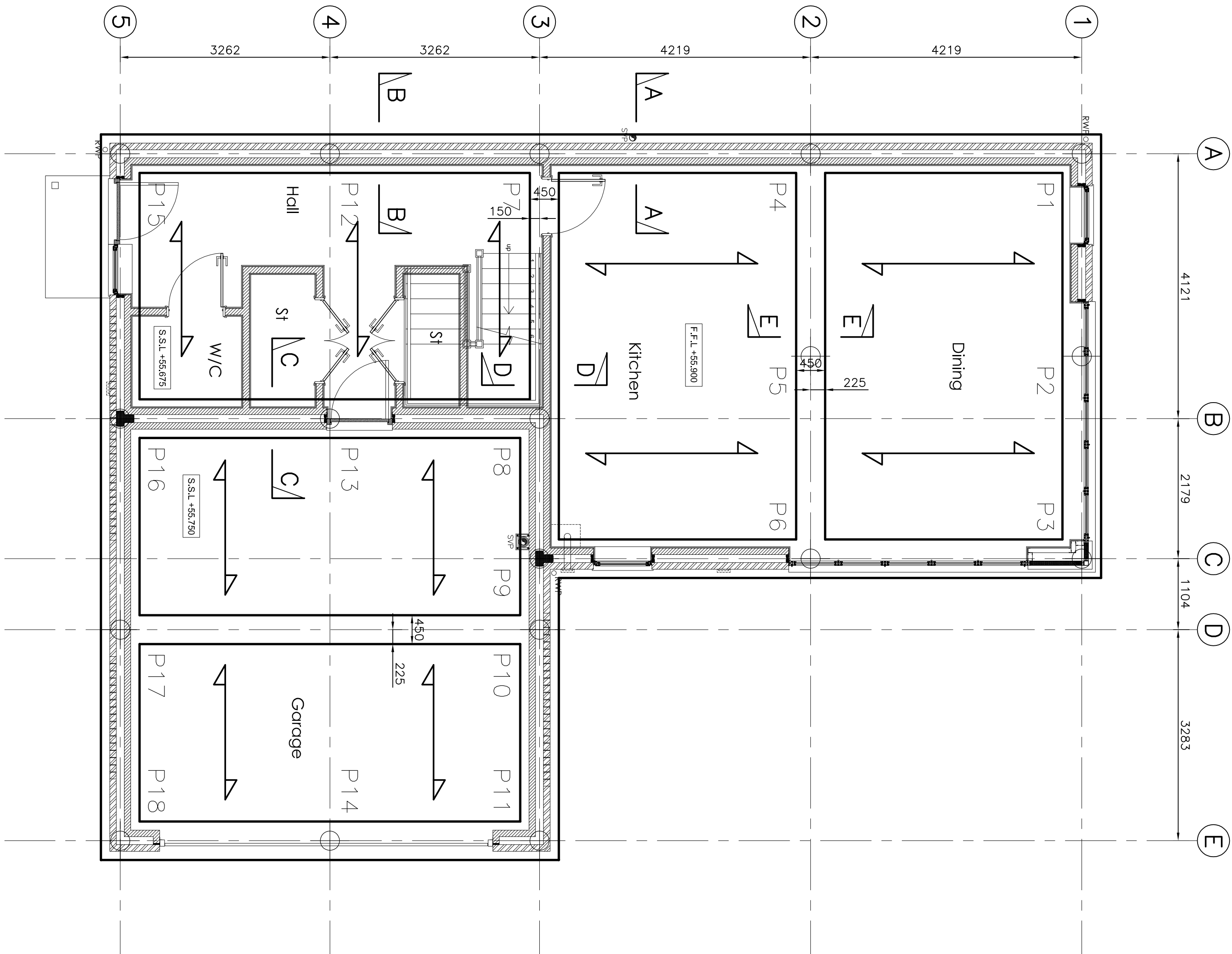
PLOT 1 GROUND BEAM LAYOUT 1:50
