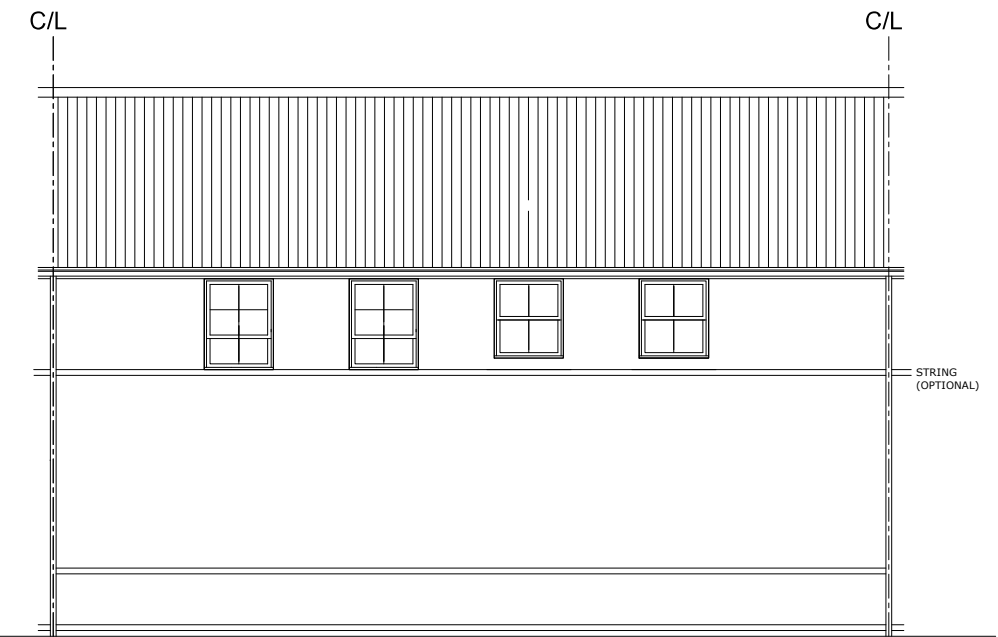
REAR ELEVATION
