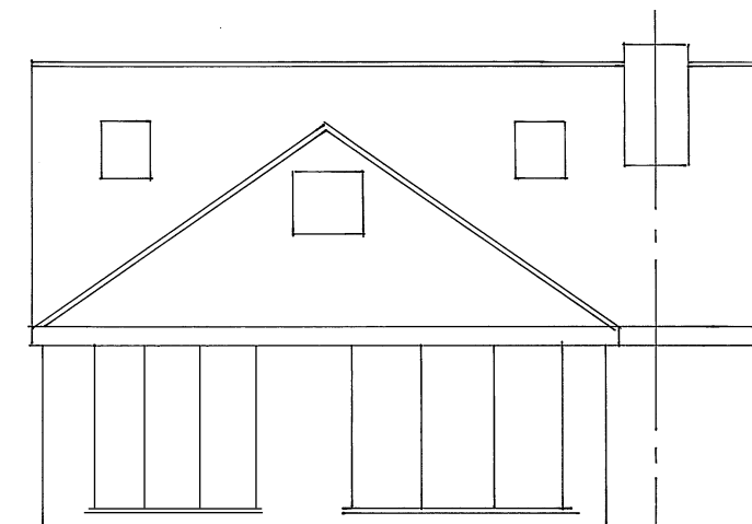
Existing NW/Rear Elevation
