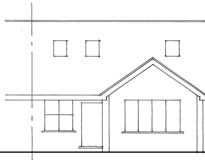
Existing SE/Front Elevation
