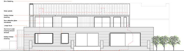
SOUTH ELEVATION
