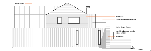
WEST ELEVATION
