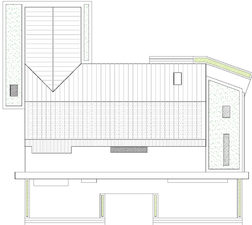
ROOF PLAN
