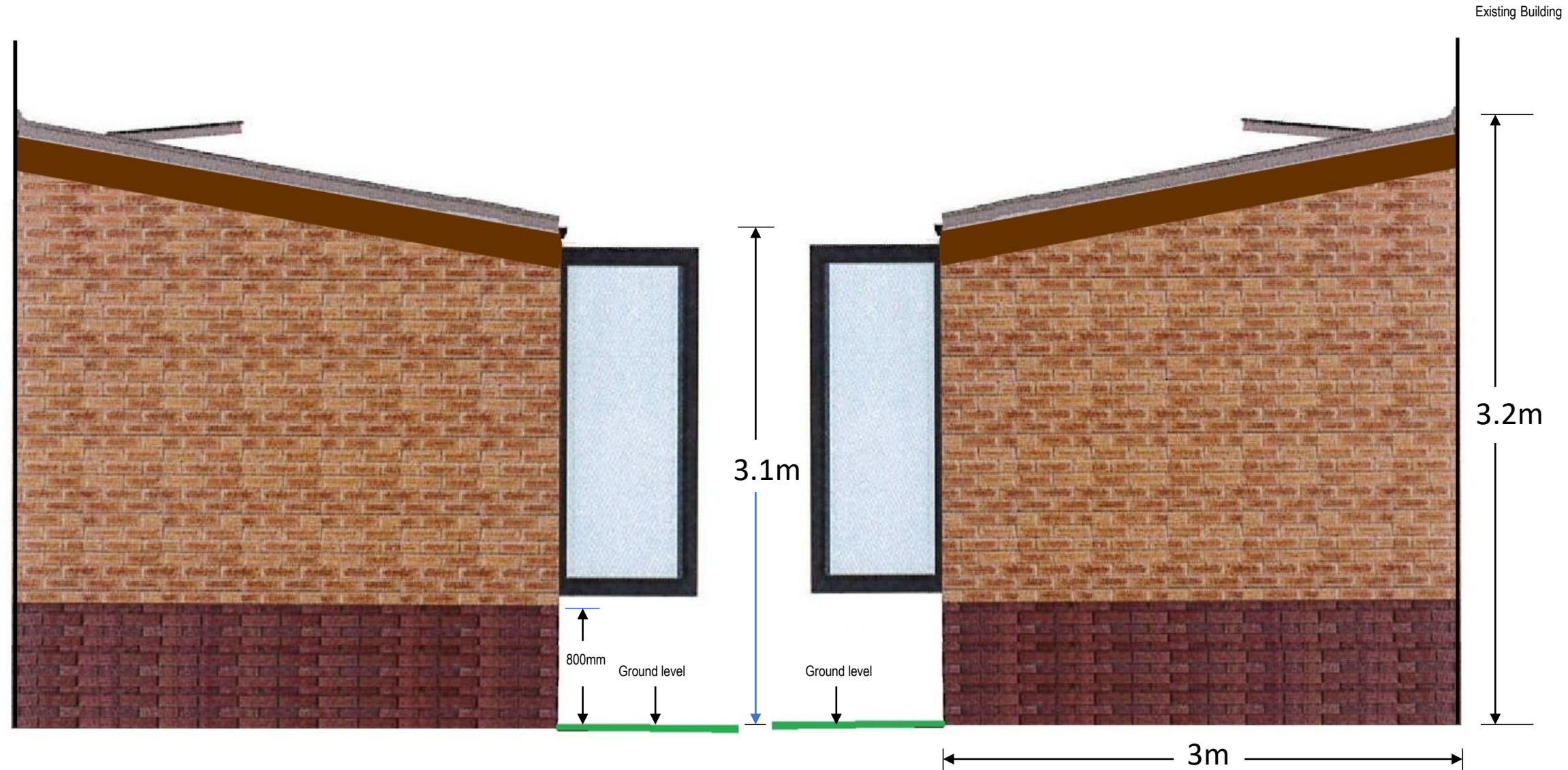
Semi detached side view
