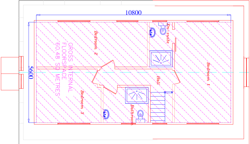
Proposed First Floor Layout
