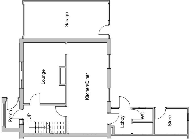
Existing Ground Floor 1 : 100
