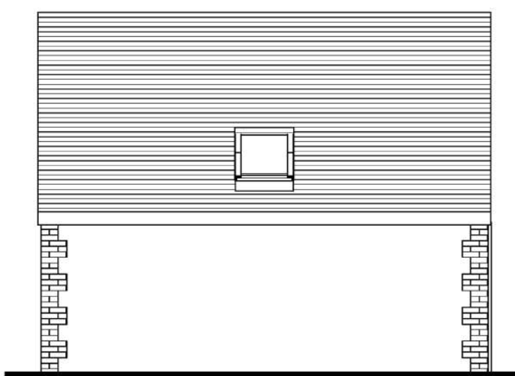
Proposed NE Elevation 1 : 100
