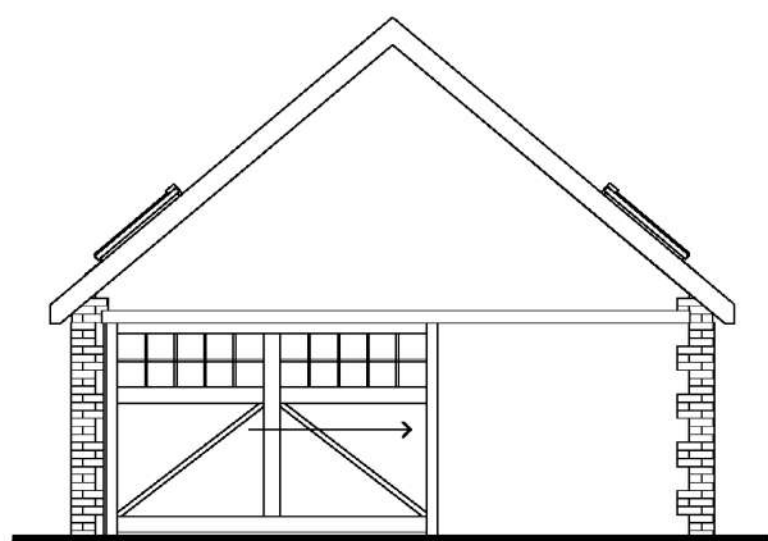
Proposed NW Elevation 1 : 100
