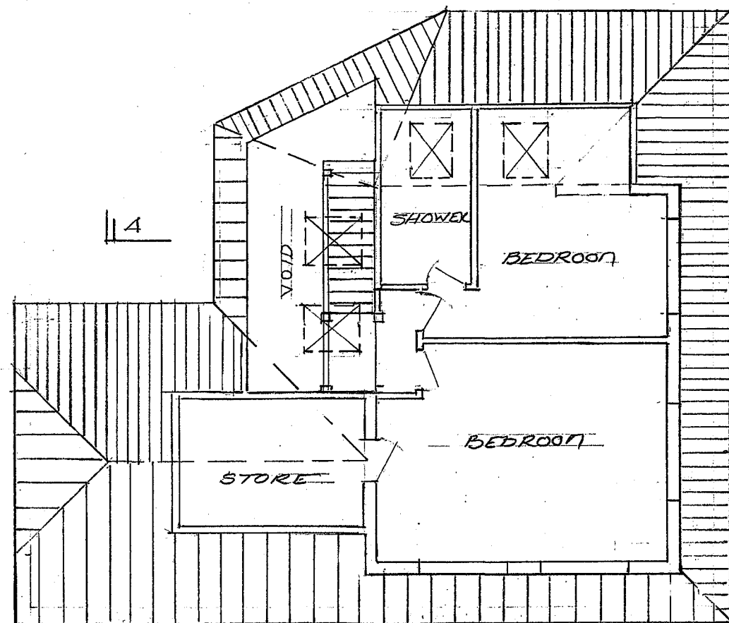
FIRST FLOOR
