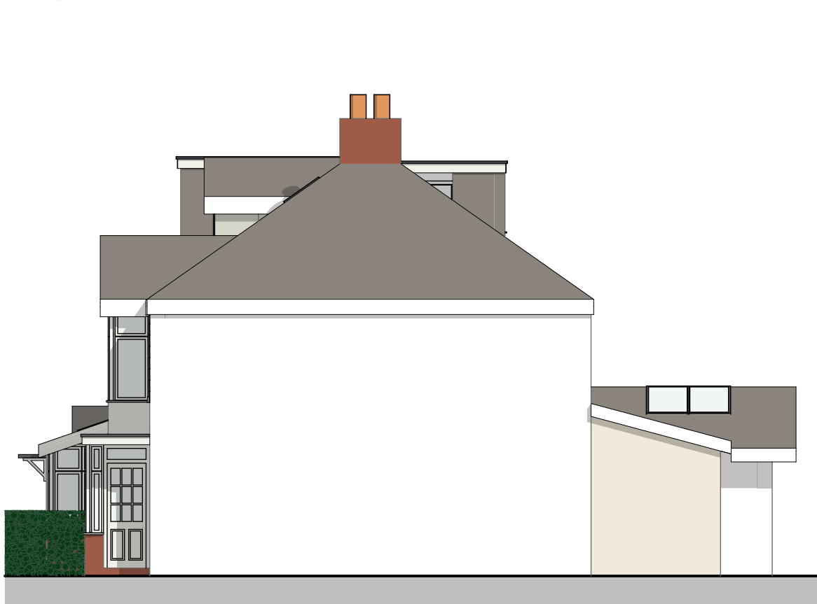
E-02 Proposed West Elevation 1:100
