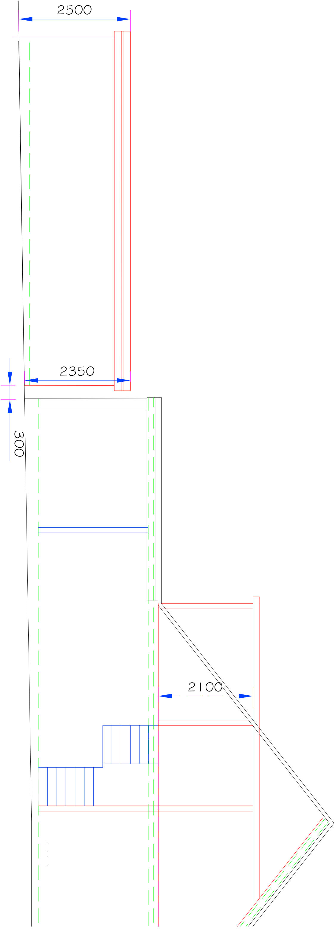
section through scale 1:50
