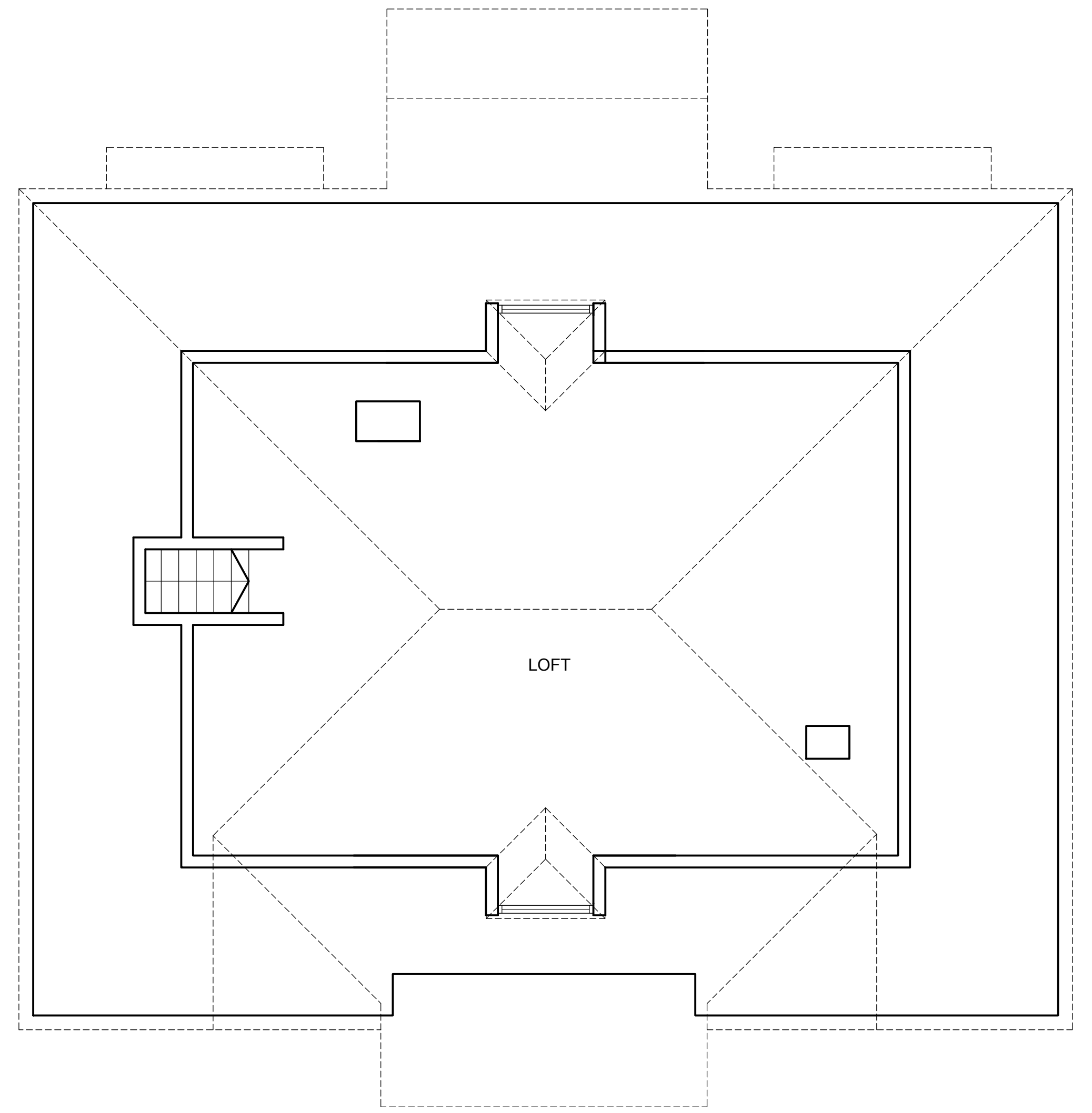
EXISTING LOFT FLOOR PLAN 1:50
