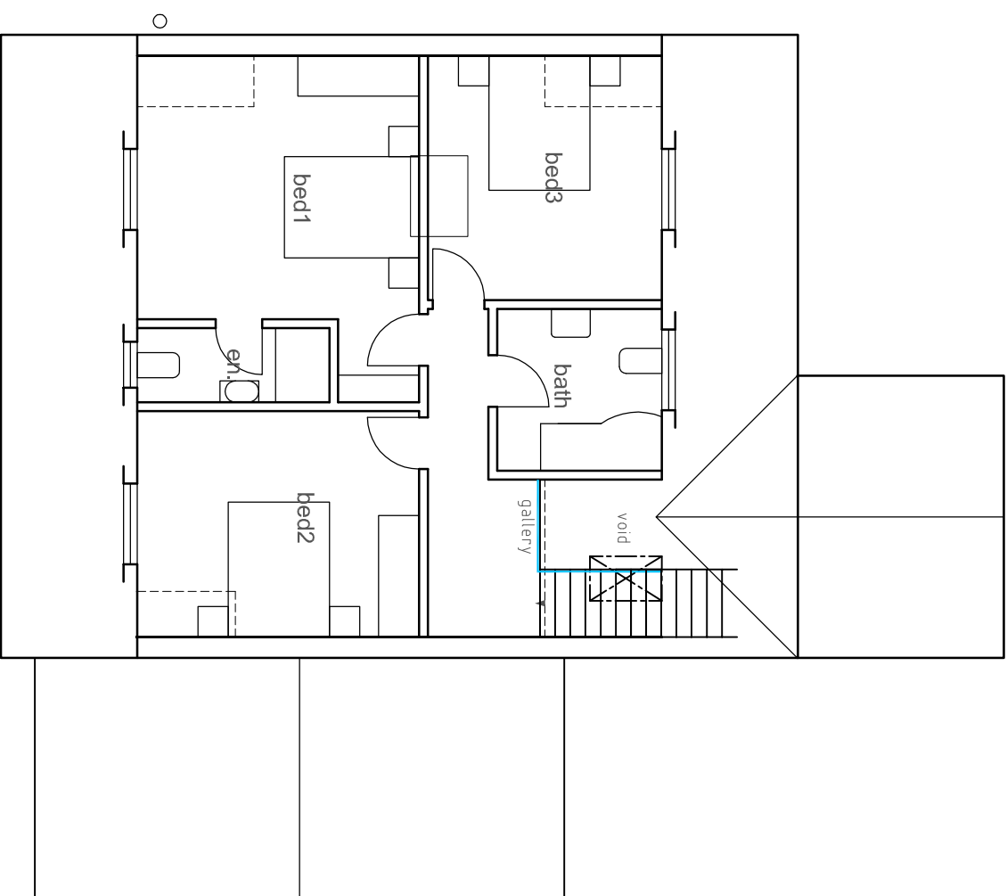
ROOF 1:100
