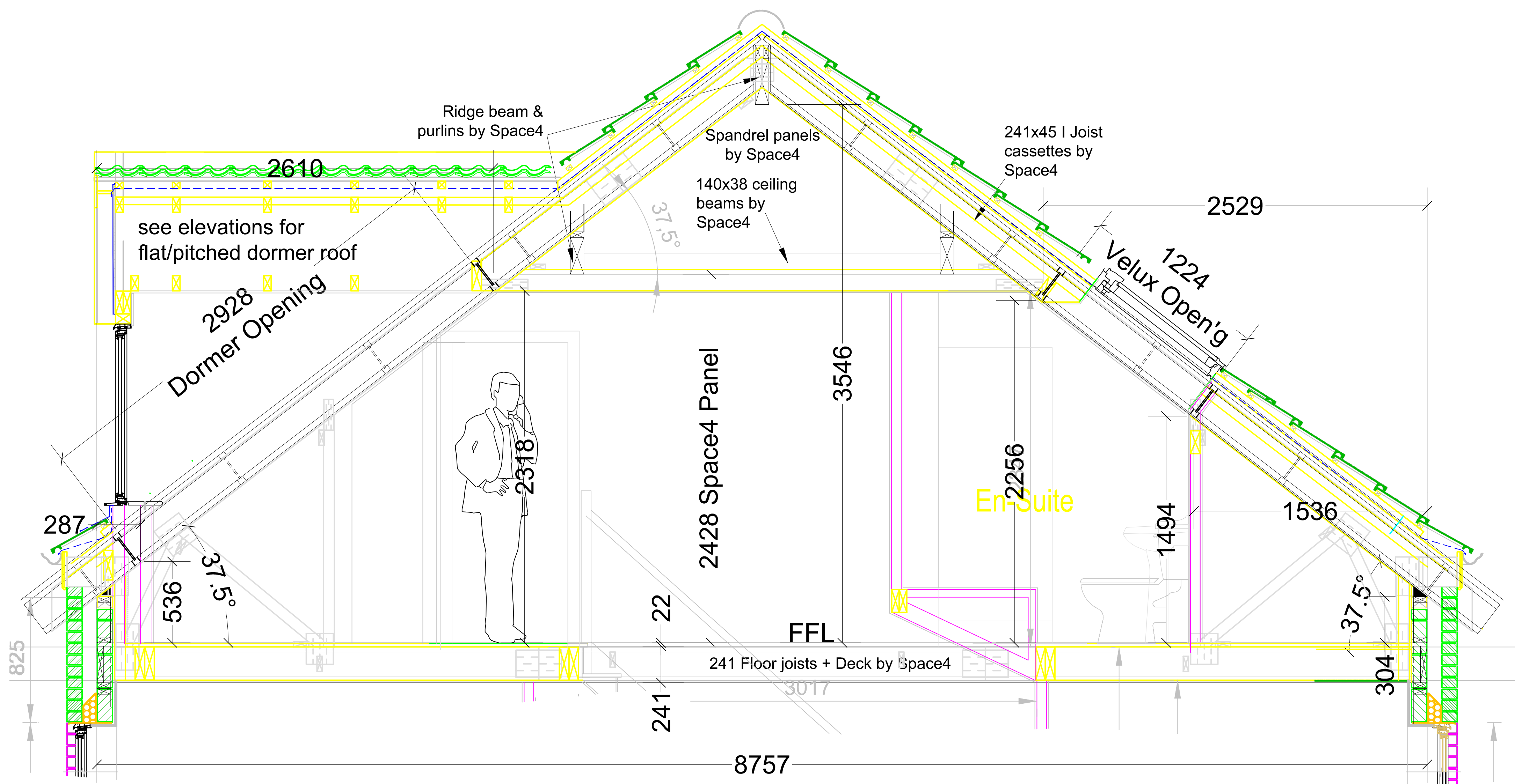
RiR SETTING OUT
