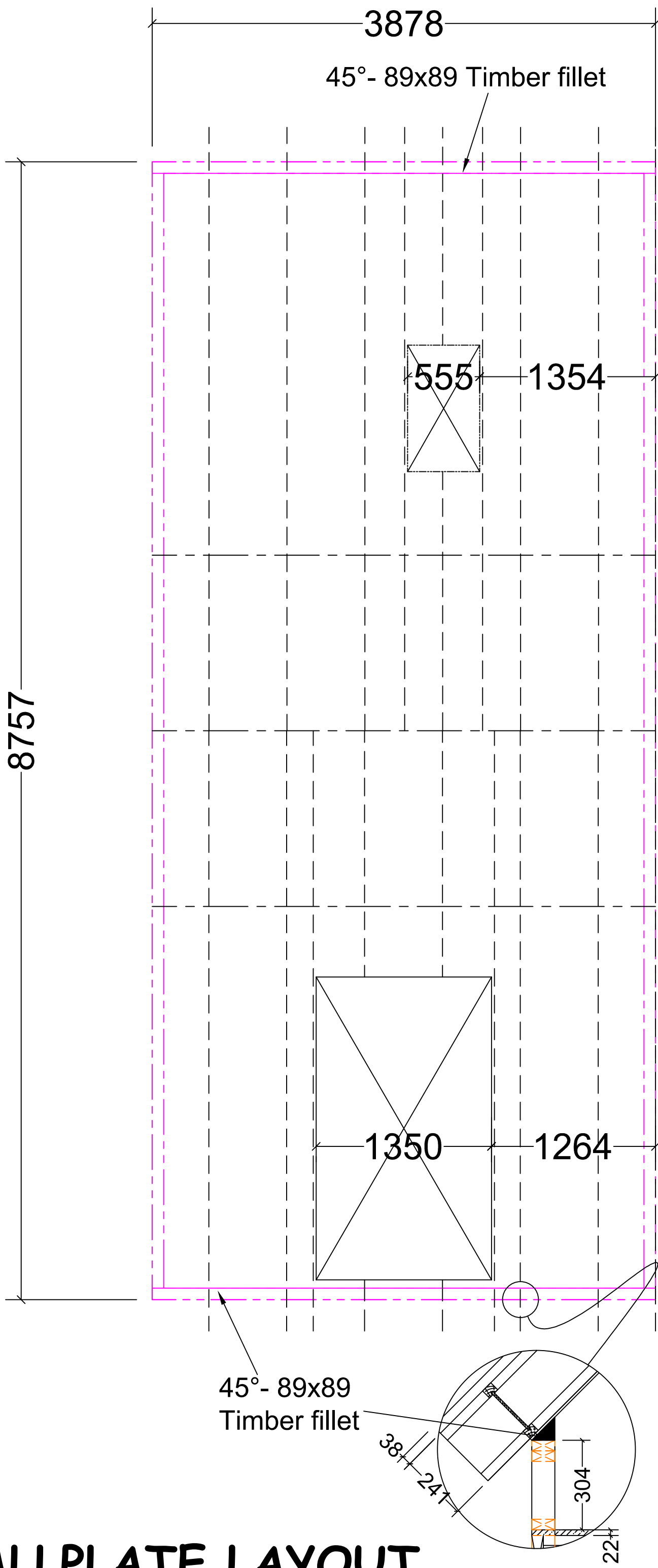
WALLPLATE LAYOUT
