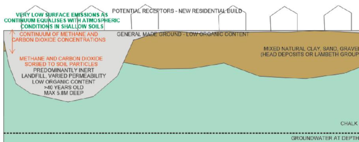
Figure 15: Ground model for Woodcroft Farm
