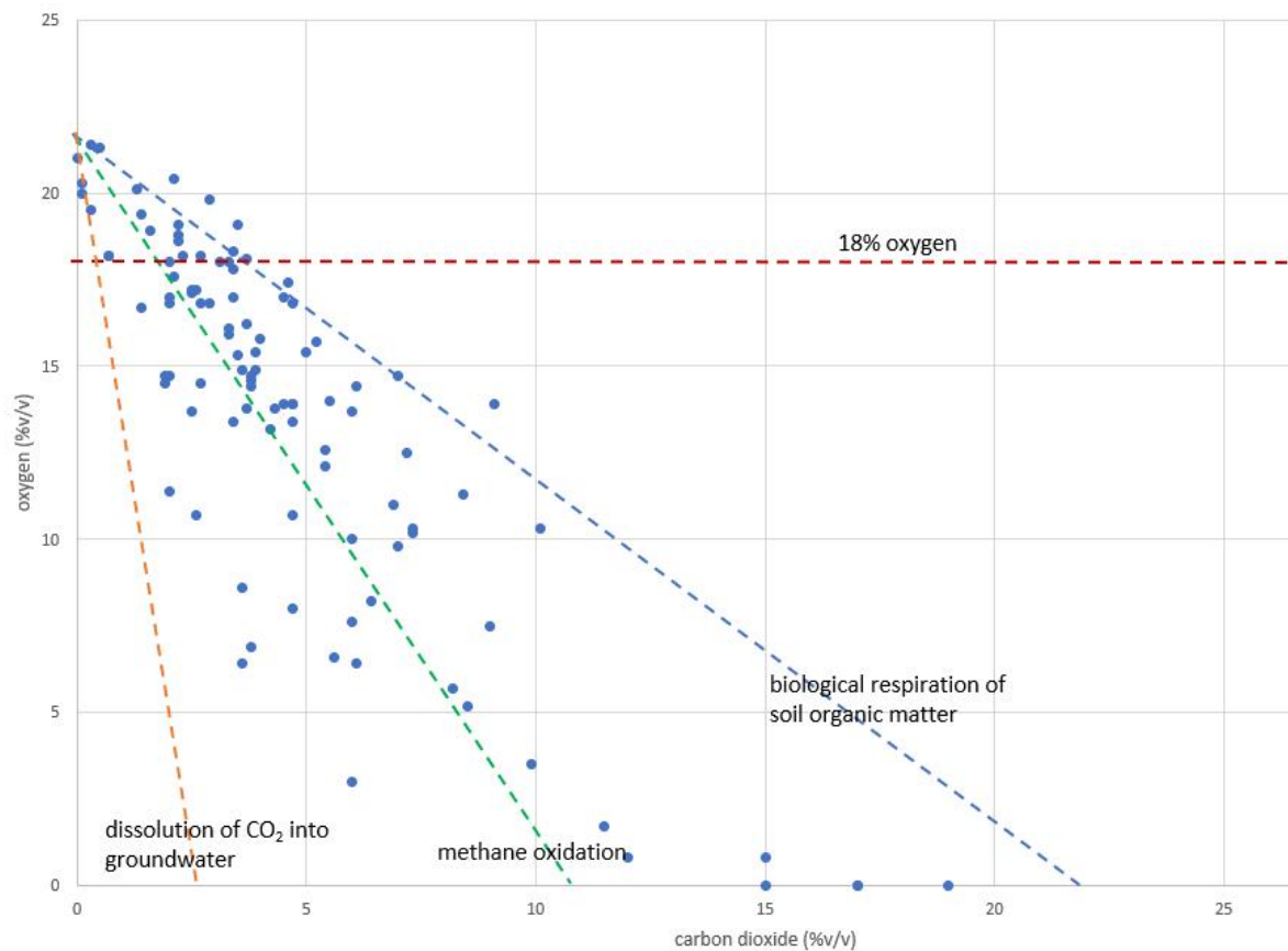
Figure 9: The relationship between oxygen and carbon dioxide
