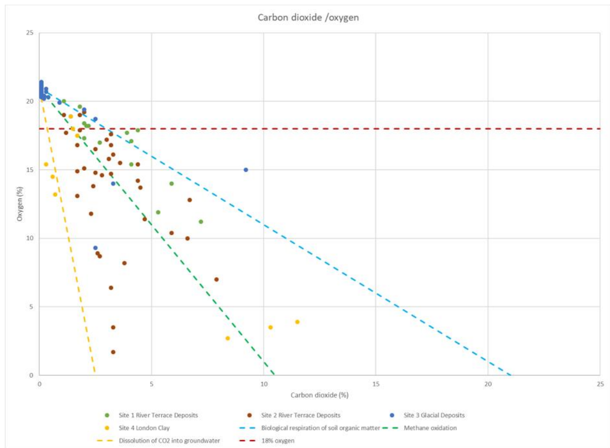
Figure 7: Carbon dioxide:oxygen relationship in natural soils
