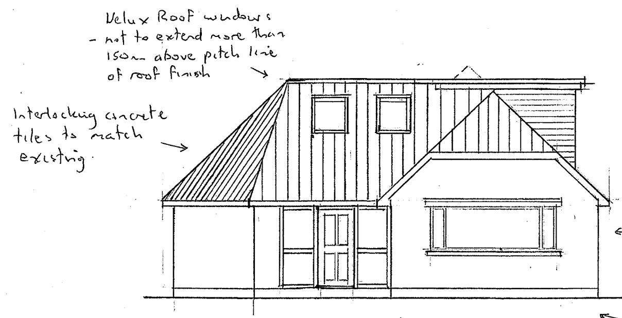
WEST ELEVATION
