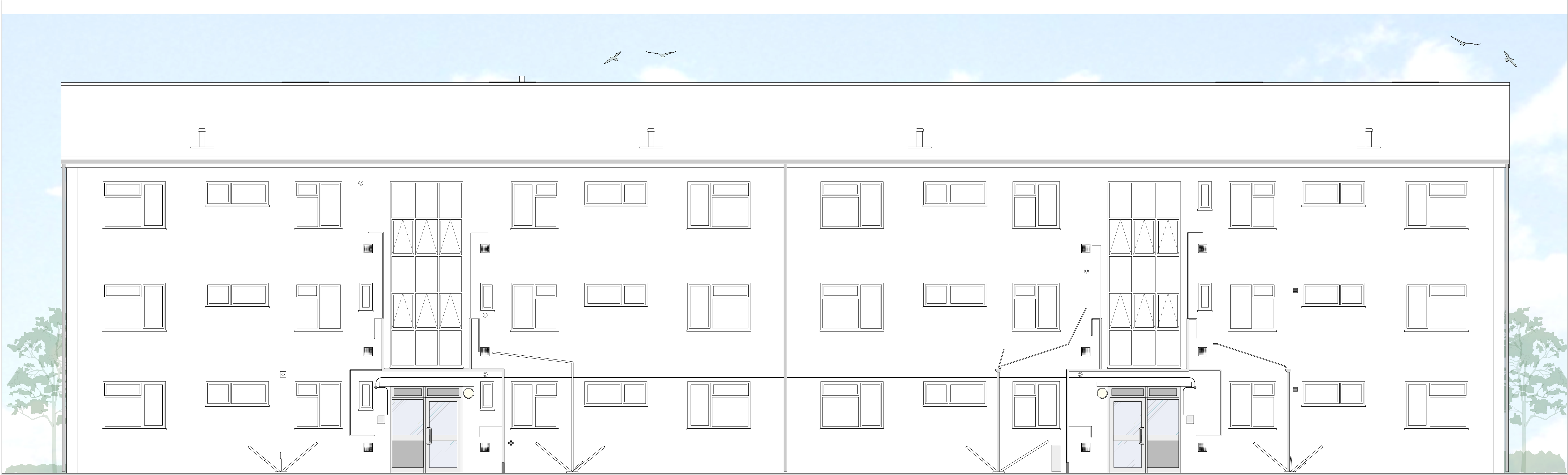
PROPOSED ELEVATION 1: FLATS 11-17A & FLATS 3-9A
