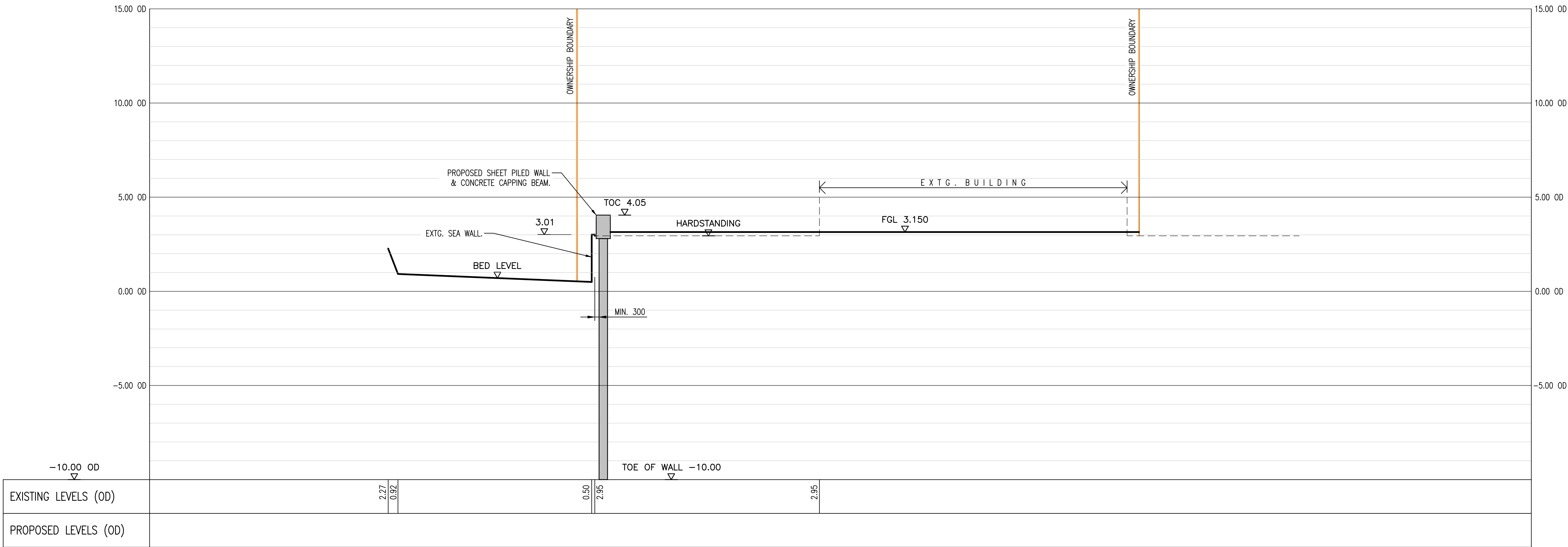
SECTION B-B. SCALE 1:125
