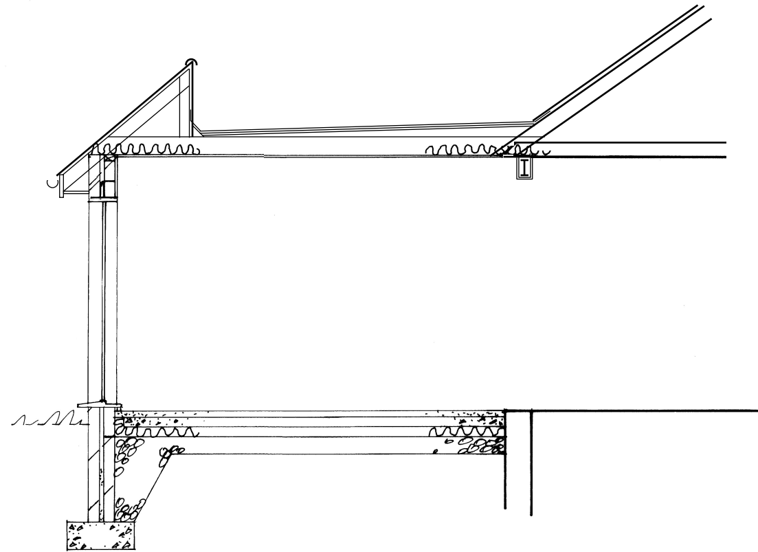
Cross-Section
