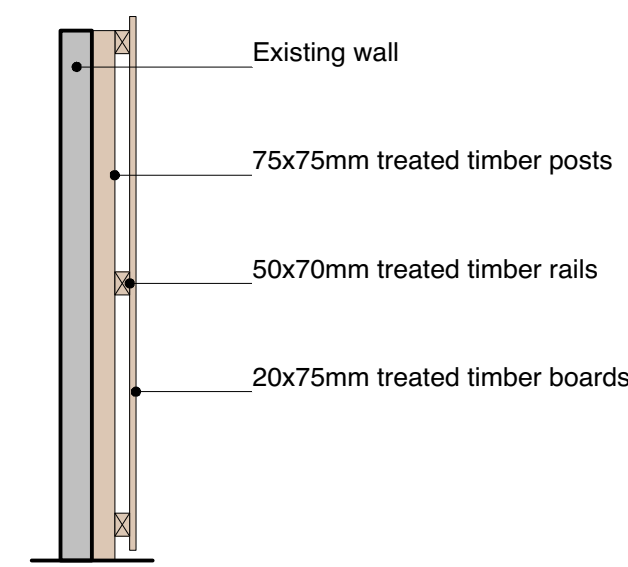
Side boundary section 1:25@A1
