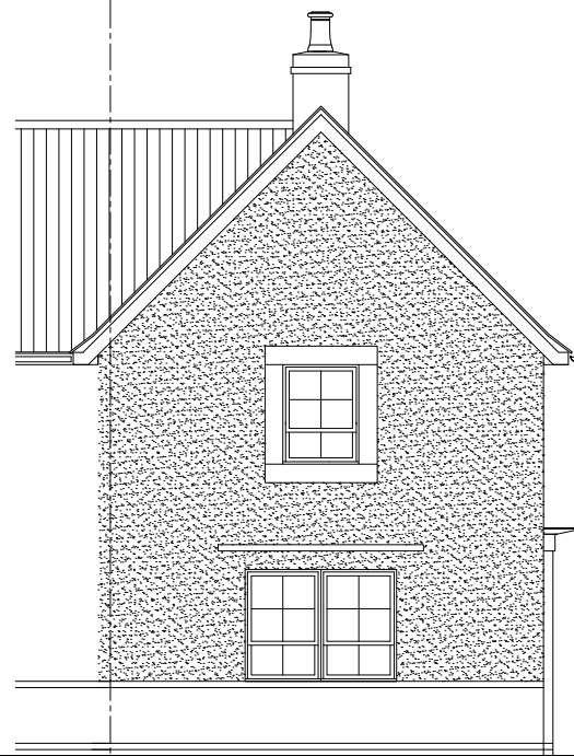
SIDE ELEVATION 1
