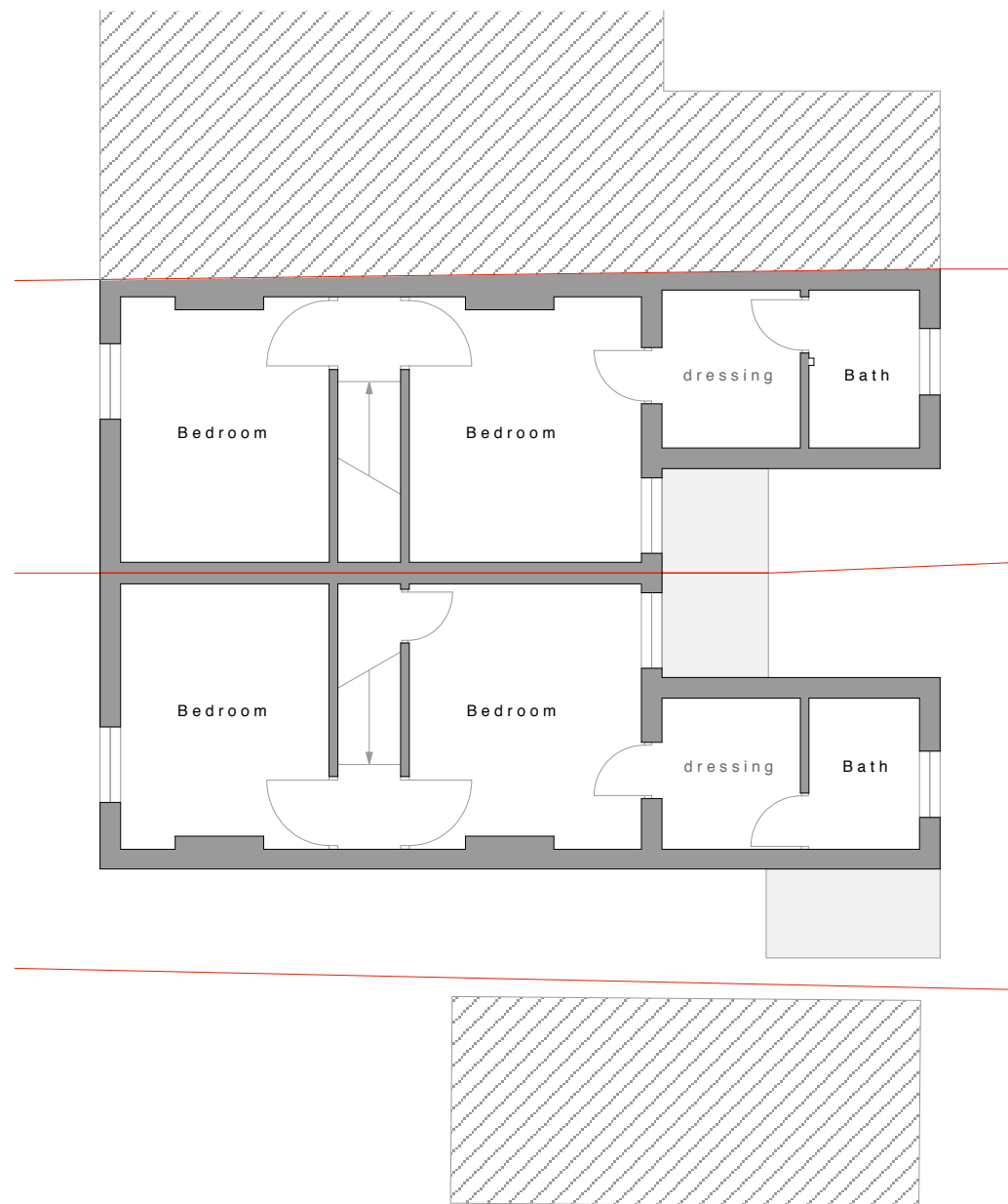
Existing First Floor Plan at 1:100 scale
