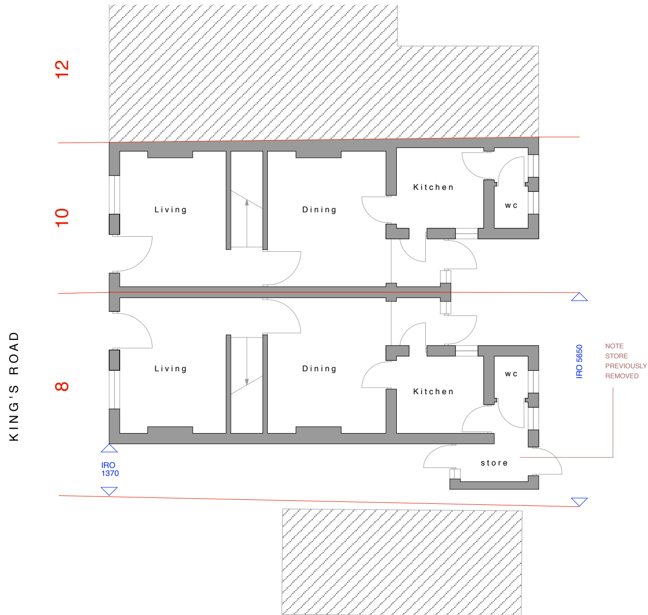
Existing Ground Floor Plan at 1:100 scale
