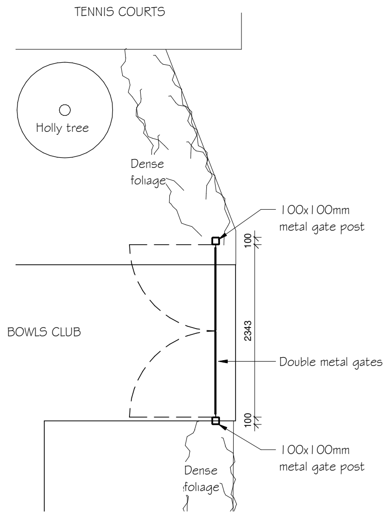
Entrance Gate - Existing Plan
