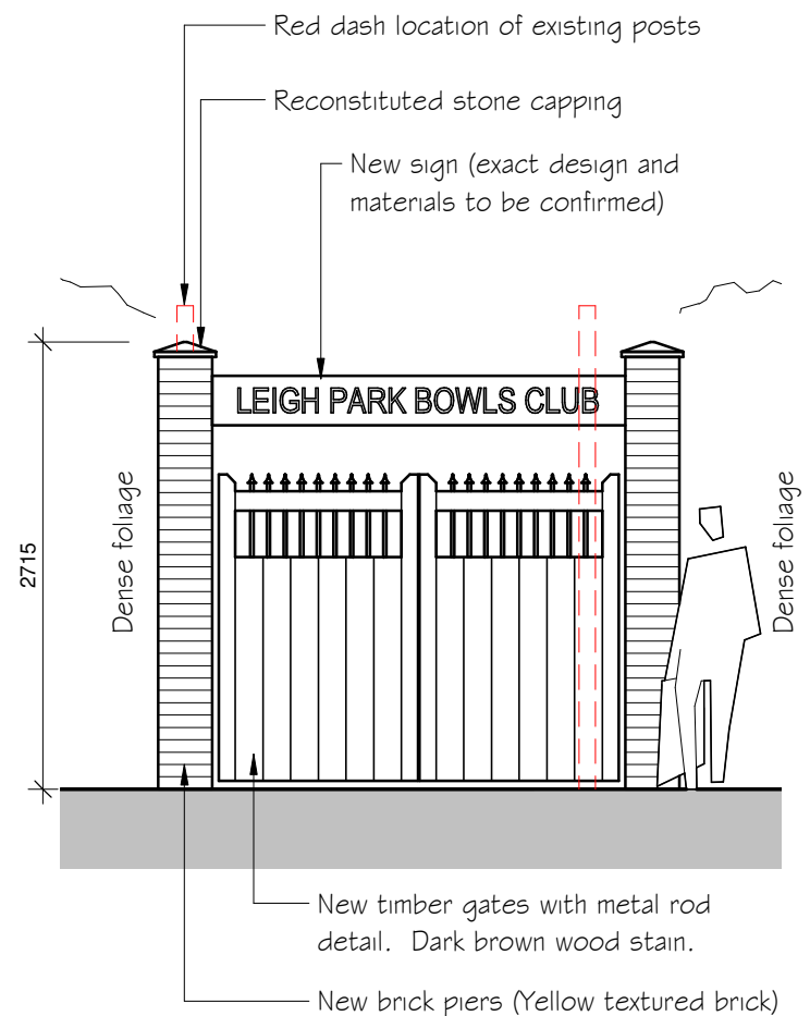
Entrance Gate - Proposed Elevation
