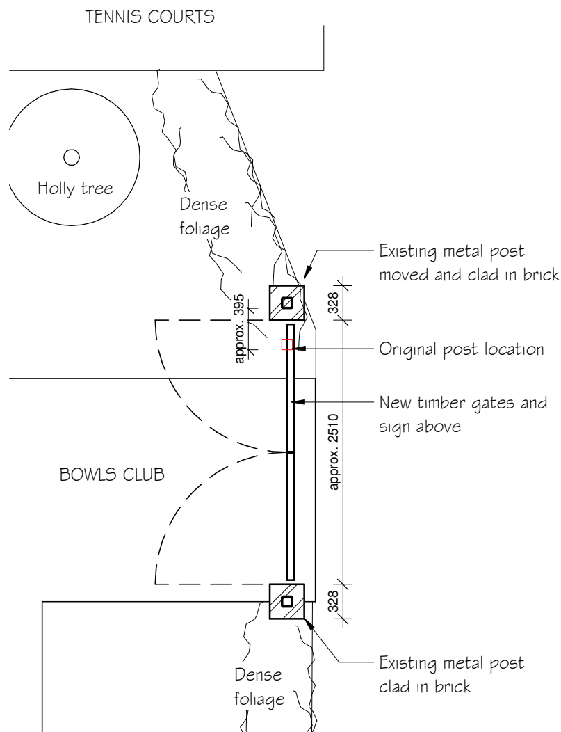
Entrance Gate - Proposed Plan
