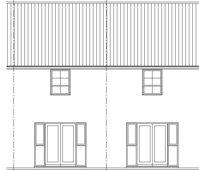
REAR ELEVATION
