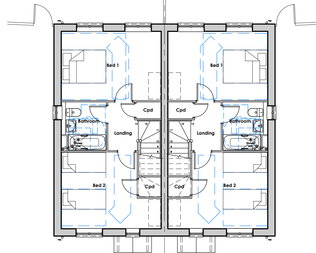
Plot 4 First Floor Layout
