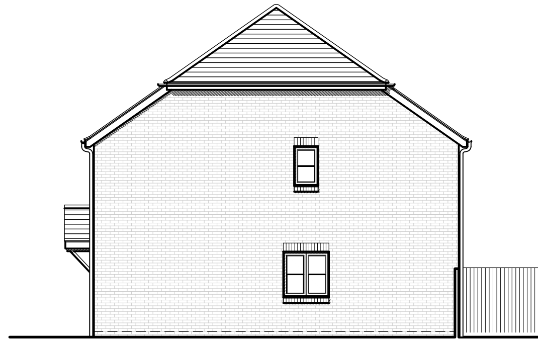
Plot 5 Side Elevation
