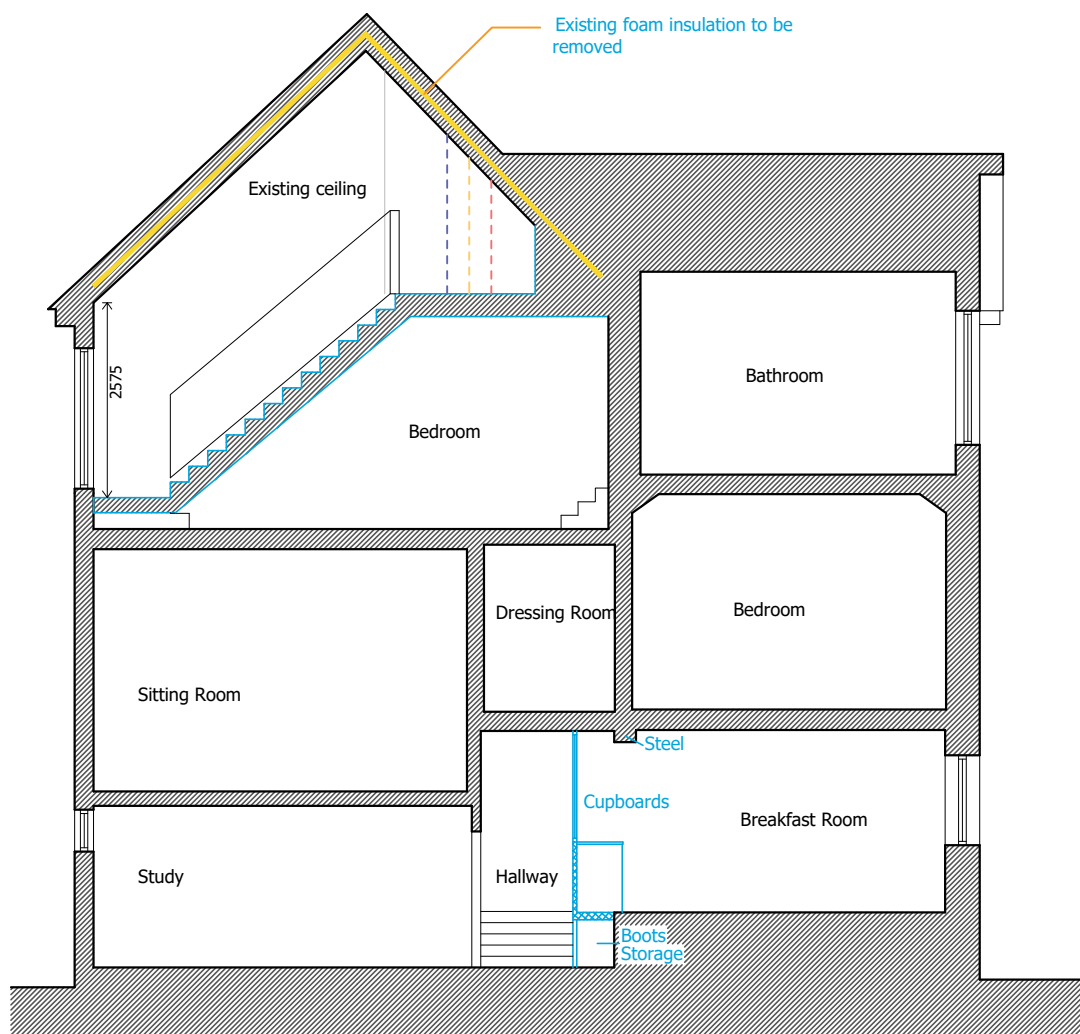
SECTION B-B 1:100
