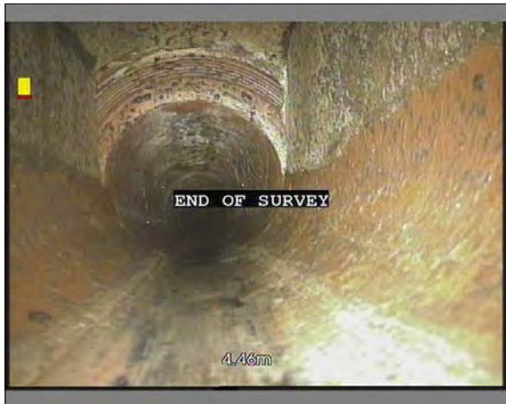
Photo: 011.JPG, VCR No.: 00007 4.46m, Manhole
