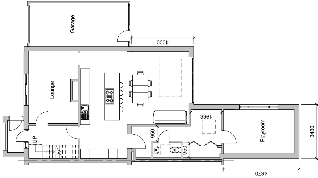
Proposed Ground Floor 1 : 100
