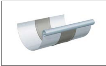
Expansion Joint short, half-round/box section, expansion element zinc-grey
