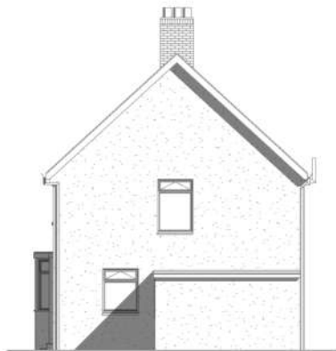
ELEVATION SIDE - SW 1 : 100
