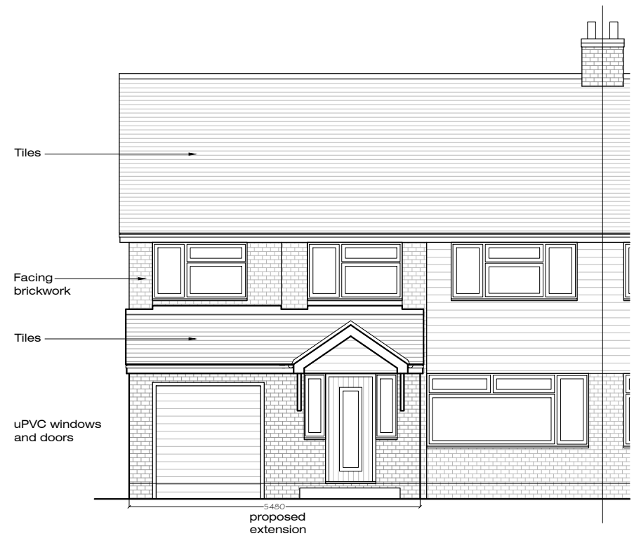
South-West (Front) Elevation - As Proposed
