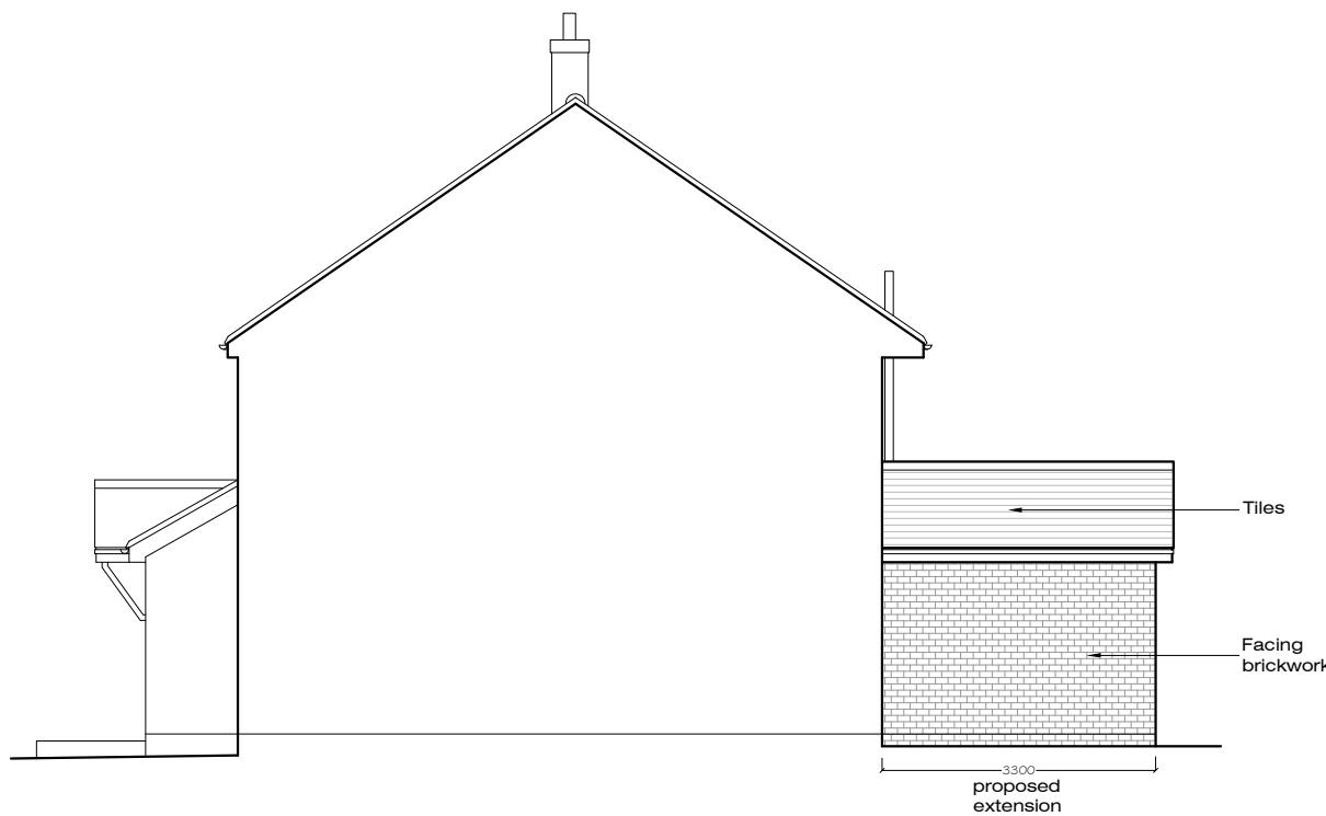
South-East (Side) Elevation - As Proposed
