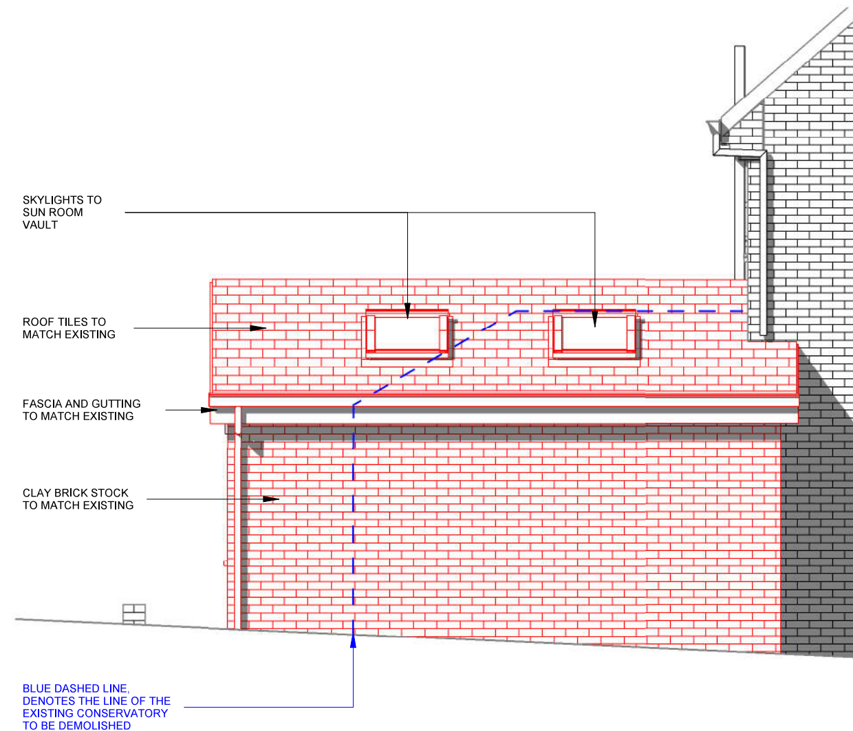
DETAILED ELEVATION SOUTH 1 : 50
