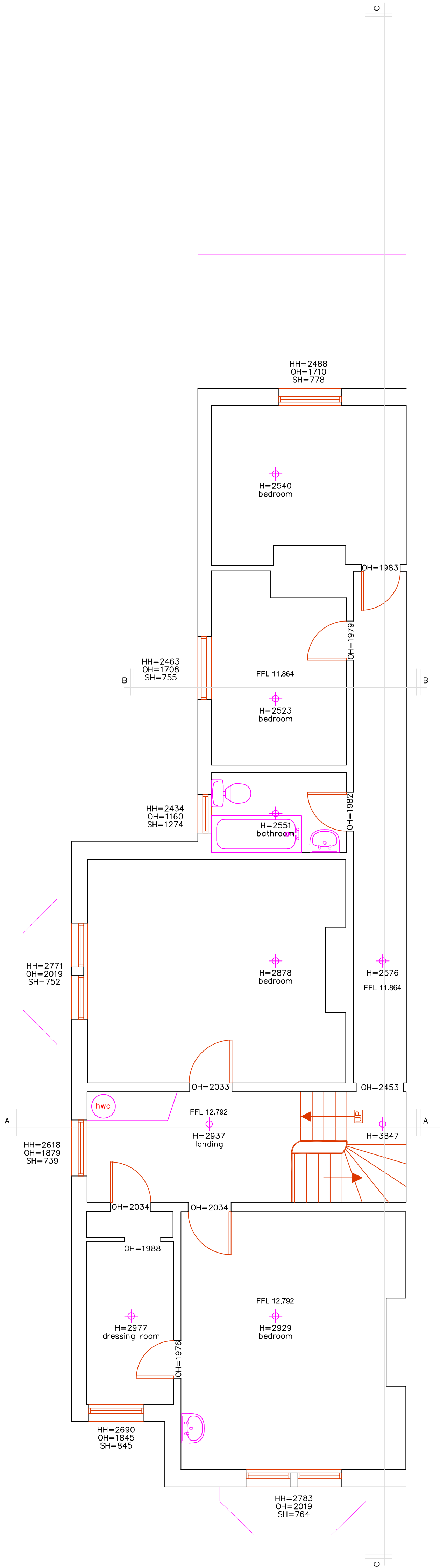
First floor plan 1:50
