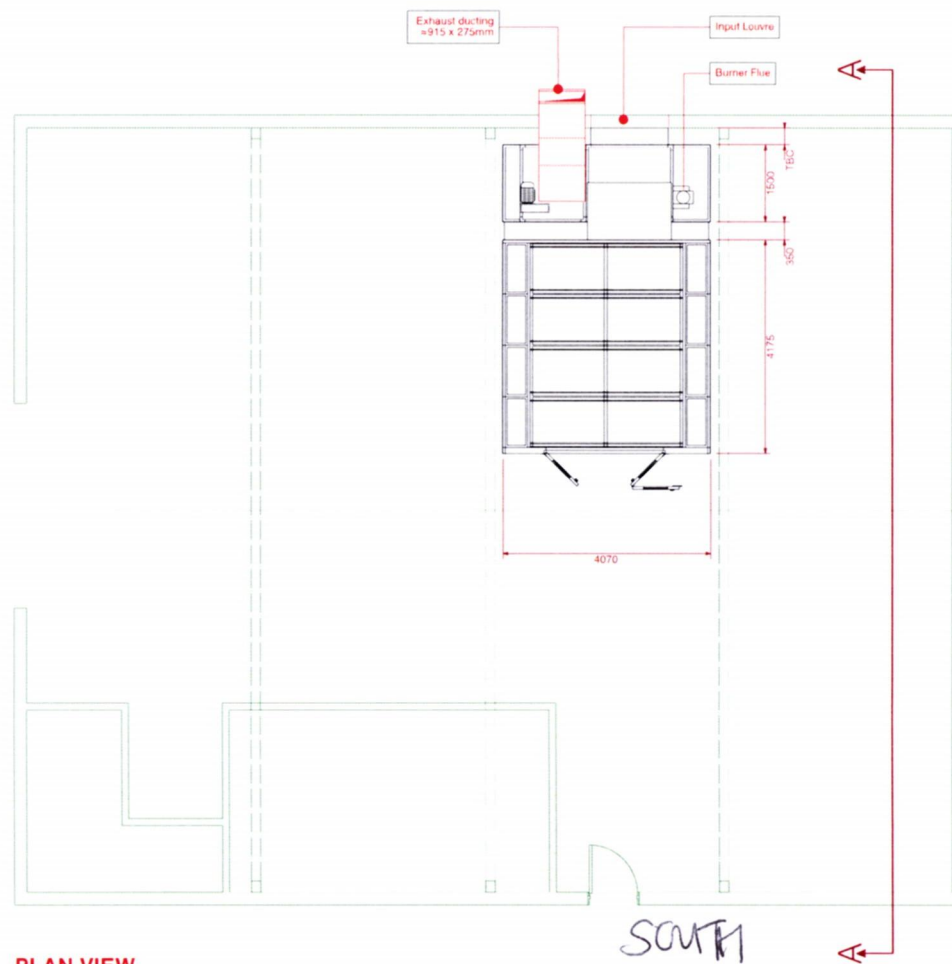
PLAN VIEW
