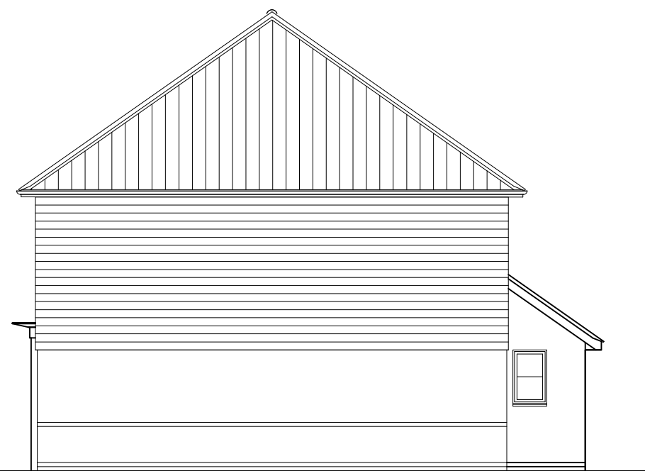
SIDE ELEVATION 2
