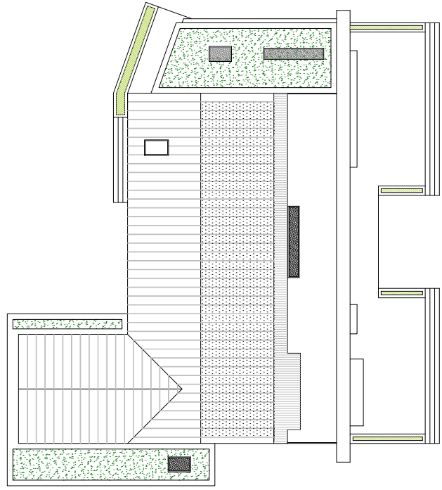
ROOF PLAN 1:100
