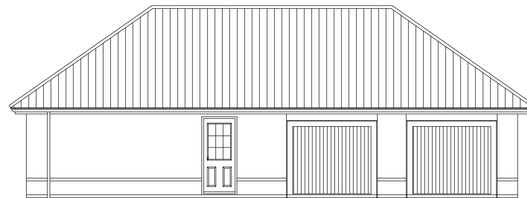
SIDE ELEVATION 2
