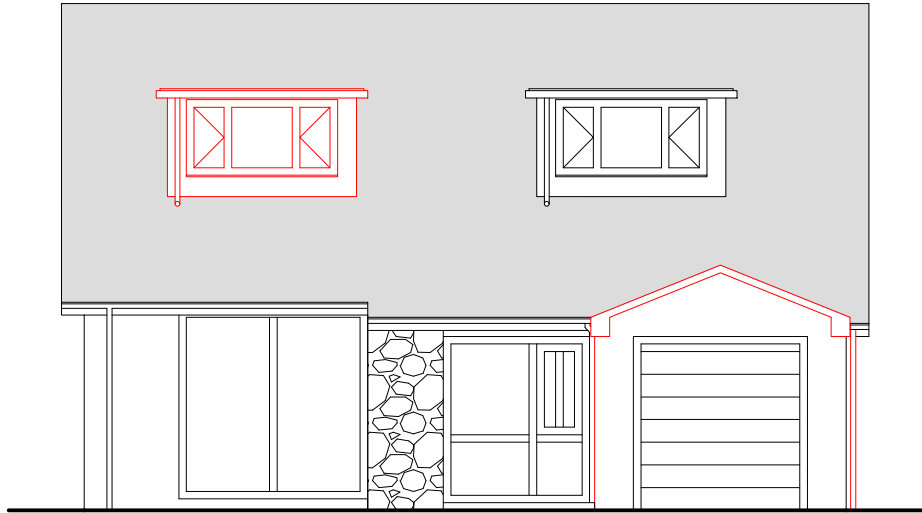
SOUTH
