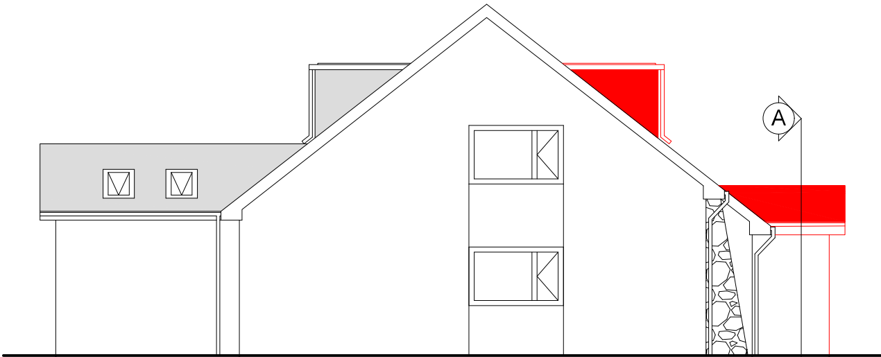
WEST
