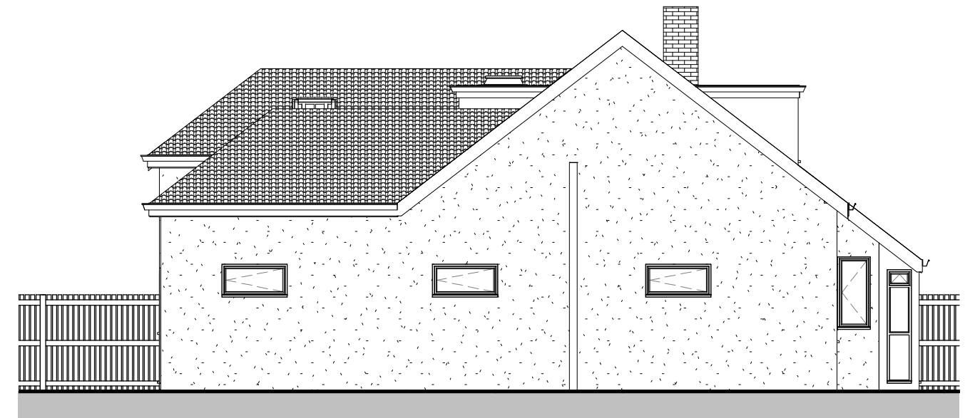
2 East Elevation 1 : 100
