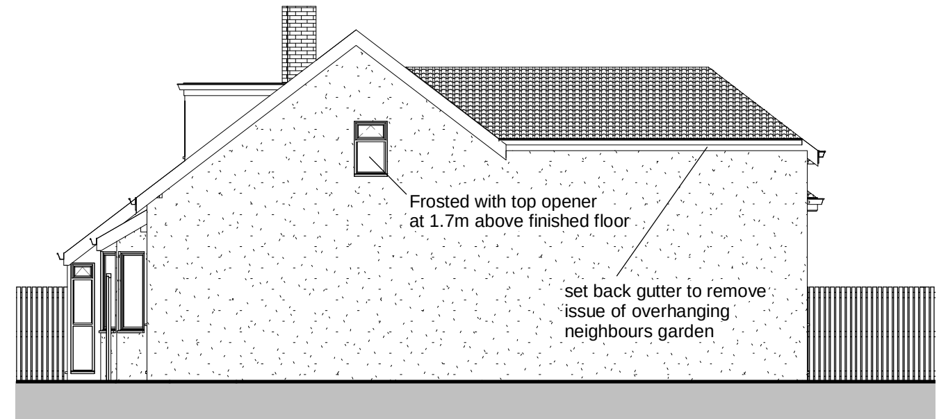
4 West Elevation 1 : 100
